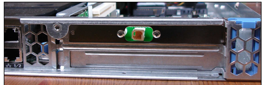
Figure 4 – External View of PCI Slot Cover Adapter Installed
