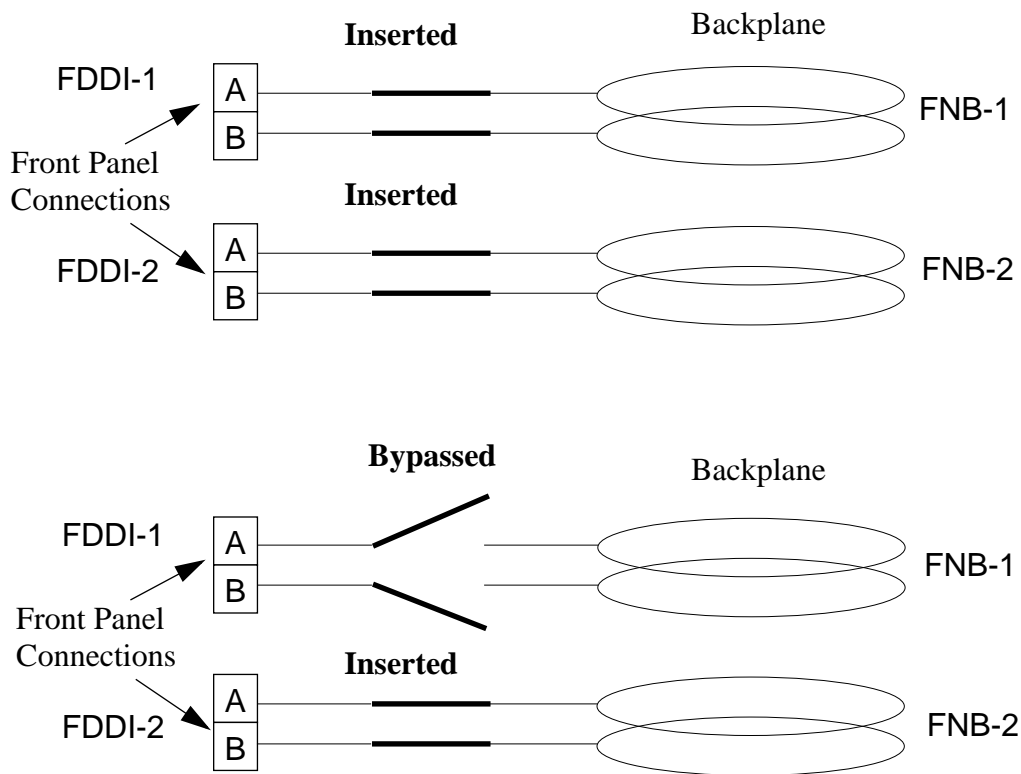
Figure 1. Front Panel Connections "Inserted" and "Bypassed"
