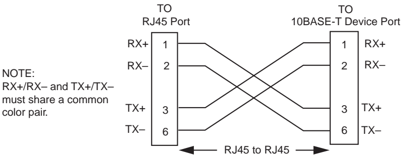
Figure 3-8 Schematic of Crossover Cable
