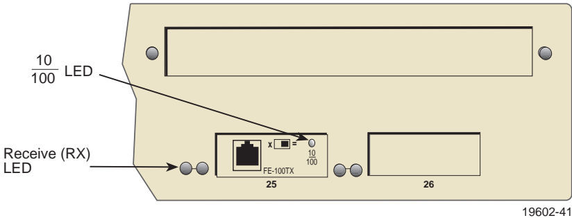
Figure 4-2 RX and 10/100 LEDs
