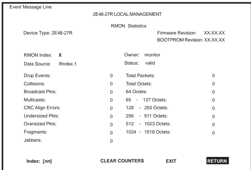
Figure 5-30 RMON Statistics Screen
