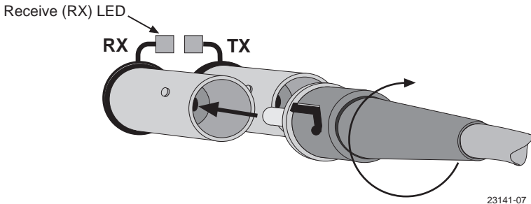
Figure 3-6 Fiber Optic Connection
