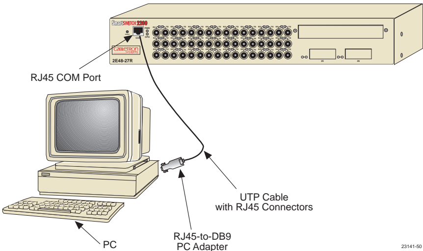
Figure 5-1 Management Terminal Connection
