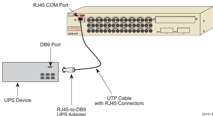
Figure 5-2 Uninterruptible Power Supply (UPS) Connection
