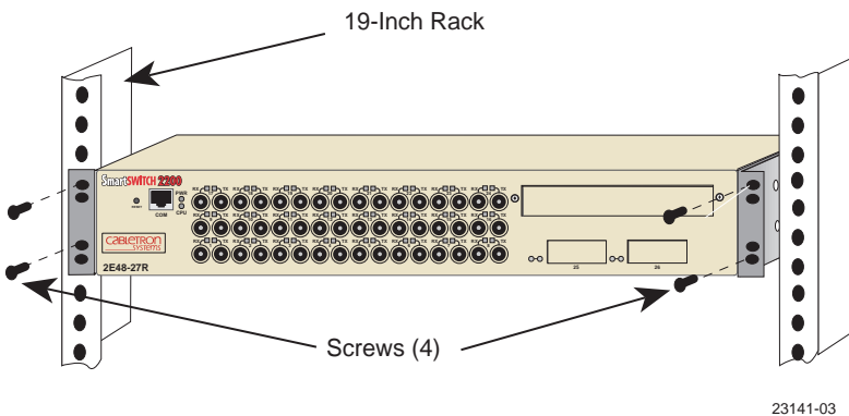
Figure 3-4 Installing the 2E4X-27R in a Rack
