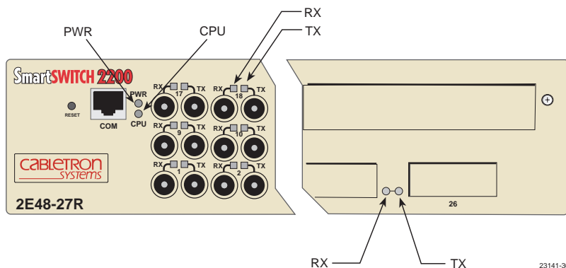
Figure 4-1 LANVIEW LEDs
