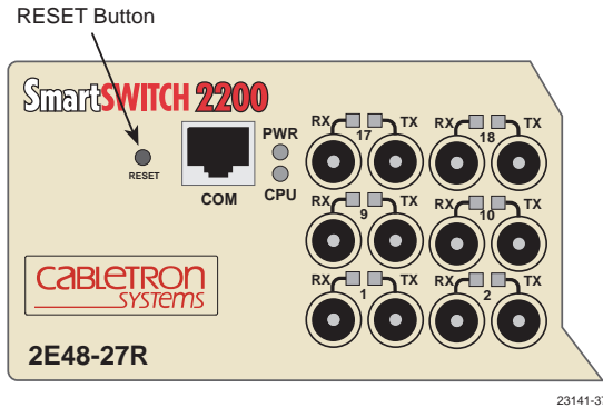
Figure 4-3 RESET Button
