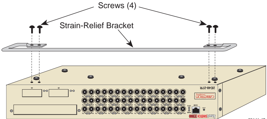
Figure 3-2 Attaching the Strain-Relief Bracket
