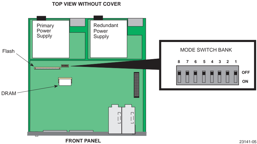
Figure C-2 2E4X-27R Mode Switch Location/Component Layout
