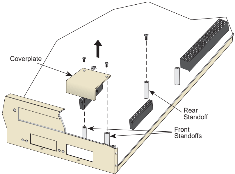
Figure C-4 Coverplate Removal
