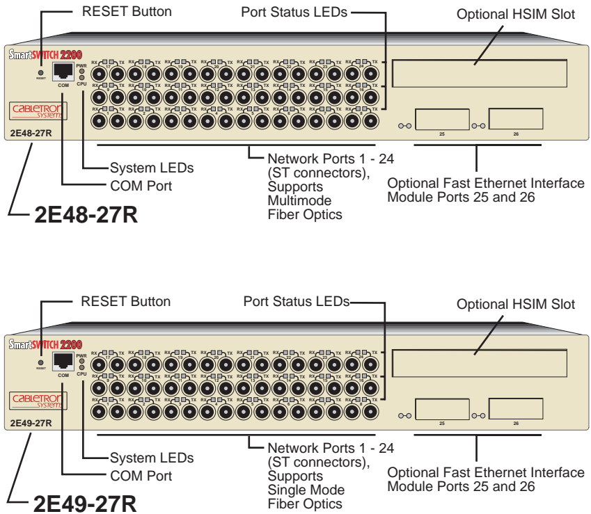
Figure 1-1 The 2E48-27R and 2E49-27R
