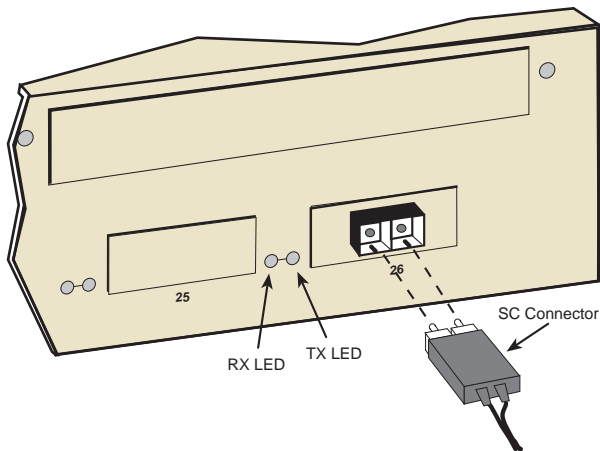
Figure 3-9 FE-100FX or FE-100F3 Port Connection
