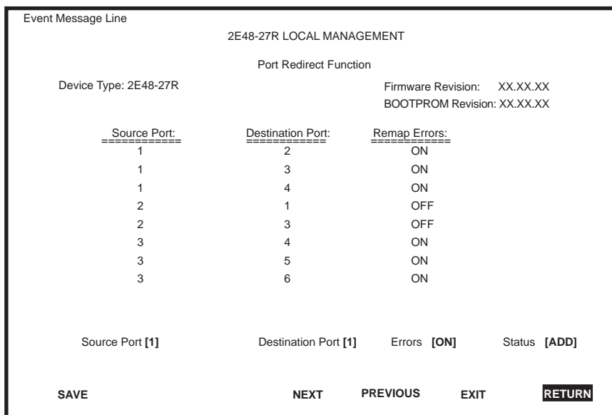
Figure 5-25 Port Redirect Function Screen
