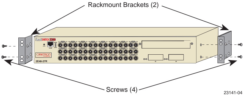
Figure 3-3 Installing the Rackmount Brackets
