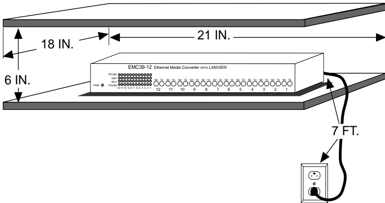
Figure 2-3 Shelf or Tabletop Installation
