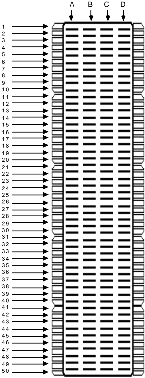
Figure B-1 Punch Down Block Pins
