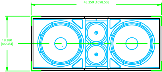
FRONT VIEW W/GRILL REMOVED
