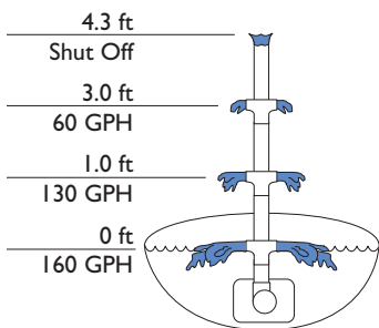
Average Performance
