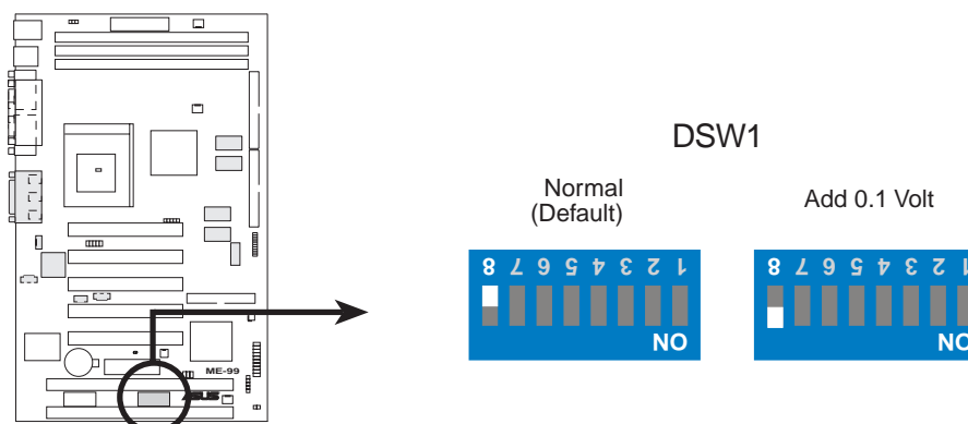
ME-99 CPU Core Voltage (Vcore) Setting
