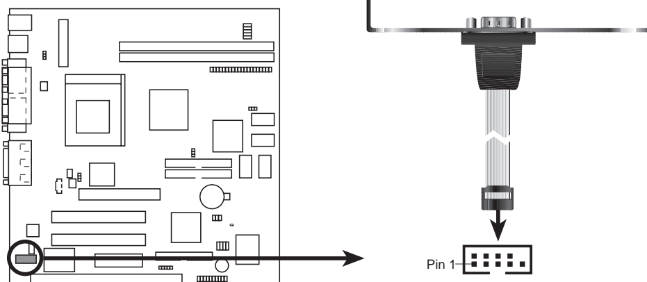
MEB-VM Serial COM 2 Header
