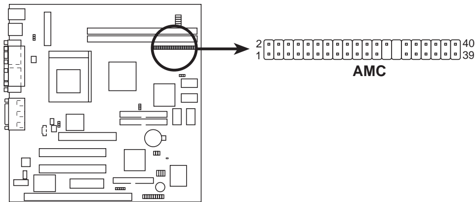
MEB-VM ATI Multimedia Channel Connector
