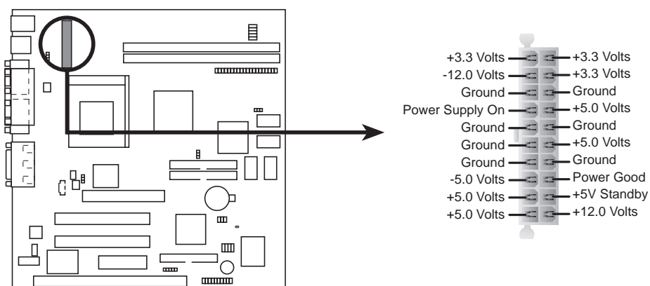
MEB-VM ATX Power Connector
