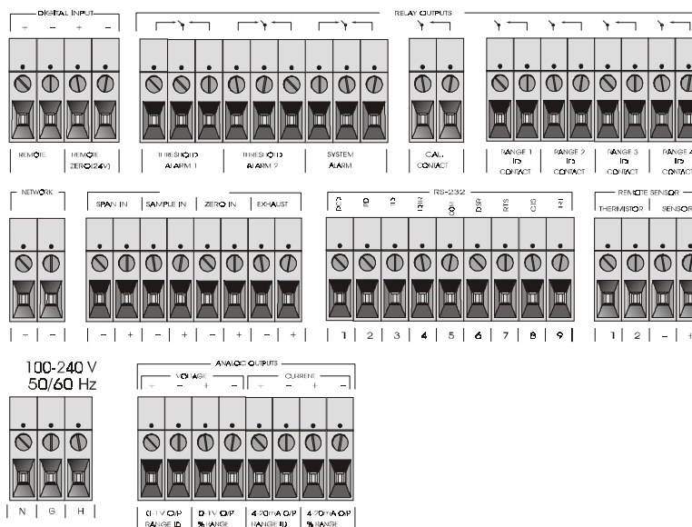
Figure 3-3: Interface Panel of the Model 3010MB Control Unit
