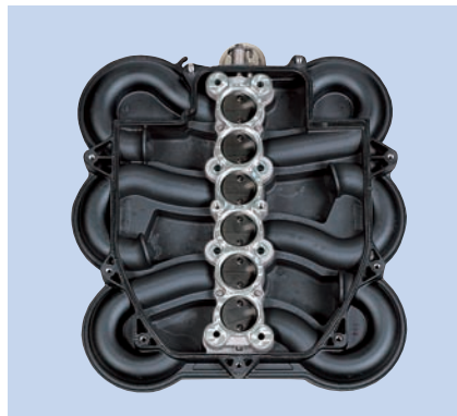
Multi-Stage Induction Module
