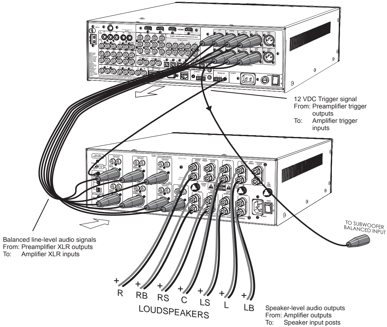
Sunfire Theater Grand Processor TGP-401
