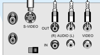
Connections Panel on VCR
